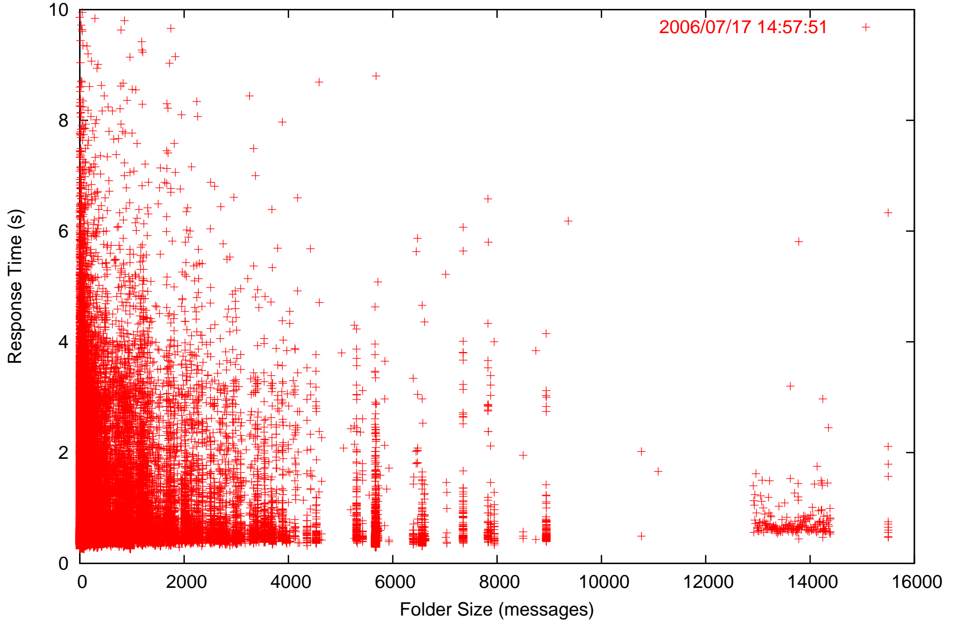
Response time Histogram for index.html from 2006/07/17 04:02:36 to 2006/07/17 14:57:51
